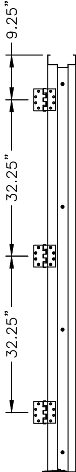
HINGE LOCATIONS 2" HEAD
