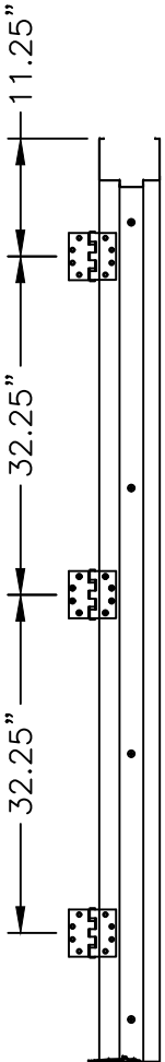
HINGE LOCATIONS 4" HEAD
