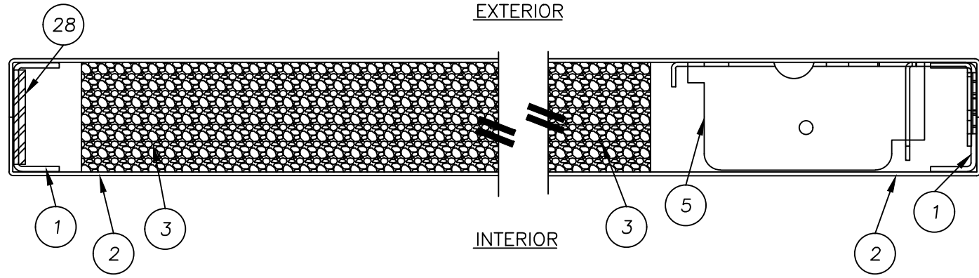
2 2 HORIZONTAL CROSS SECTION
