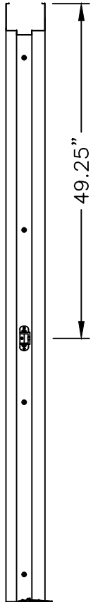
STRIKE PLATE LOCATION 4" HEAD
