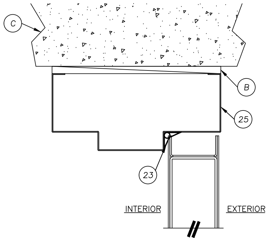
2 6 VERTICAL CROSS SECTION @ HEAD
