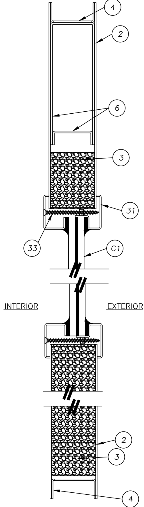
1 2 VERTICAL CROSS SECTION
